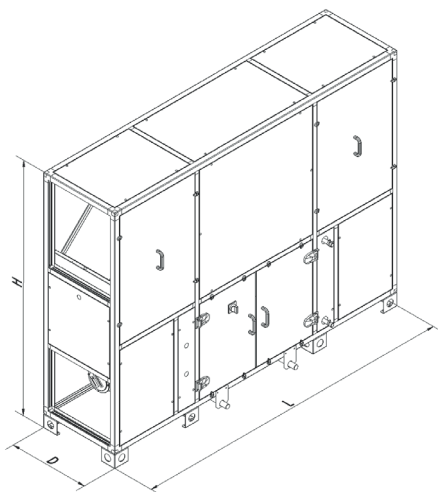
RPE VERTICAL LAYOUT WITHOUT EXTERNAL MODULE
