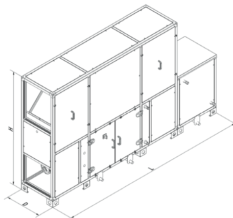
RPE VERTICAL LAYOUT WITH EXTERNAL MODULE: (ME)
